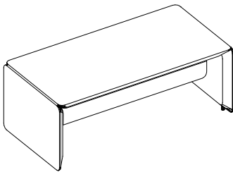
Modesty front for slab-end legs For table top width 1800, 2000, 2200 mm
